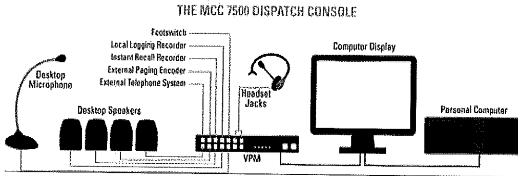
Figure 1 - 3: MCC 7500 Dispatch Console Components
